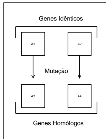
Figura 2.4 – Genes hom logos
